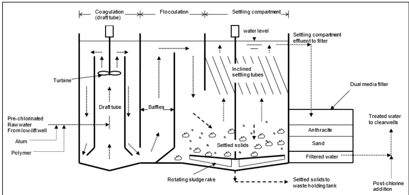
Figure 1: Sandhurst Shores Package Treatment Process Schematic
