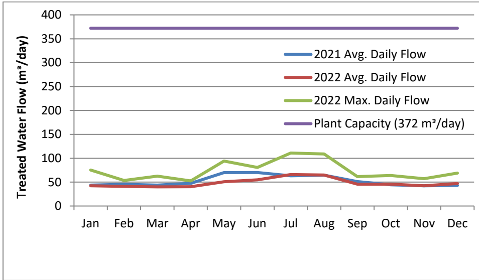
Figure 2: Monthly treated water flow trends for 2021 and 2022.
